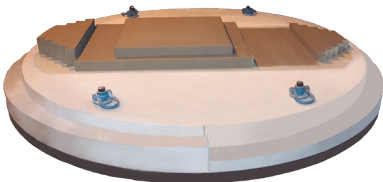
PRE-CAST LADLE BOTTOM ZONED FOR OPTIMIZED PERFORMANCE
